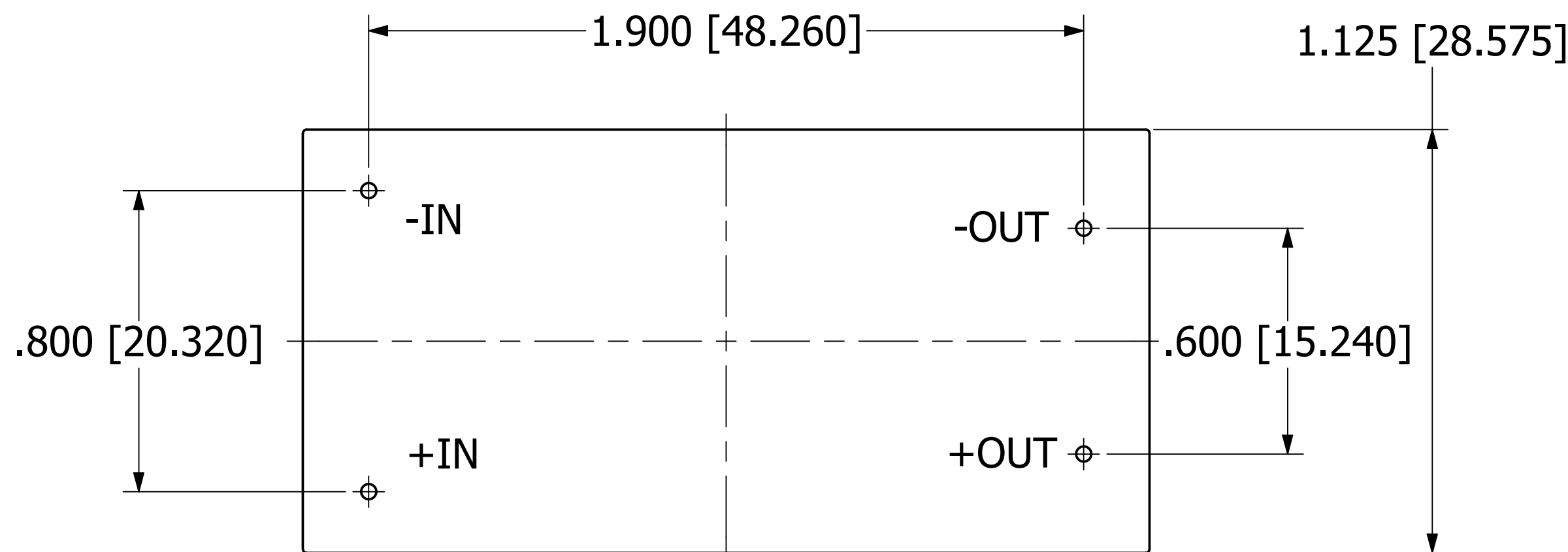
BOTTOM VIEW
